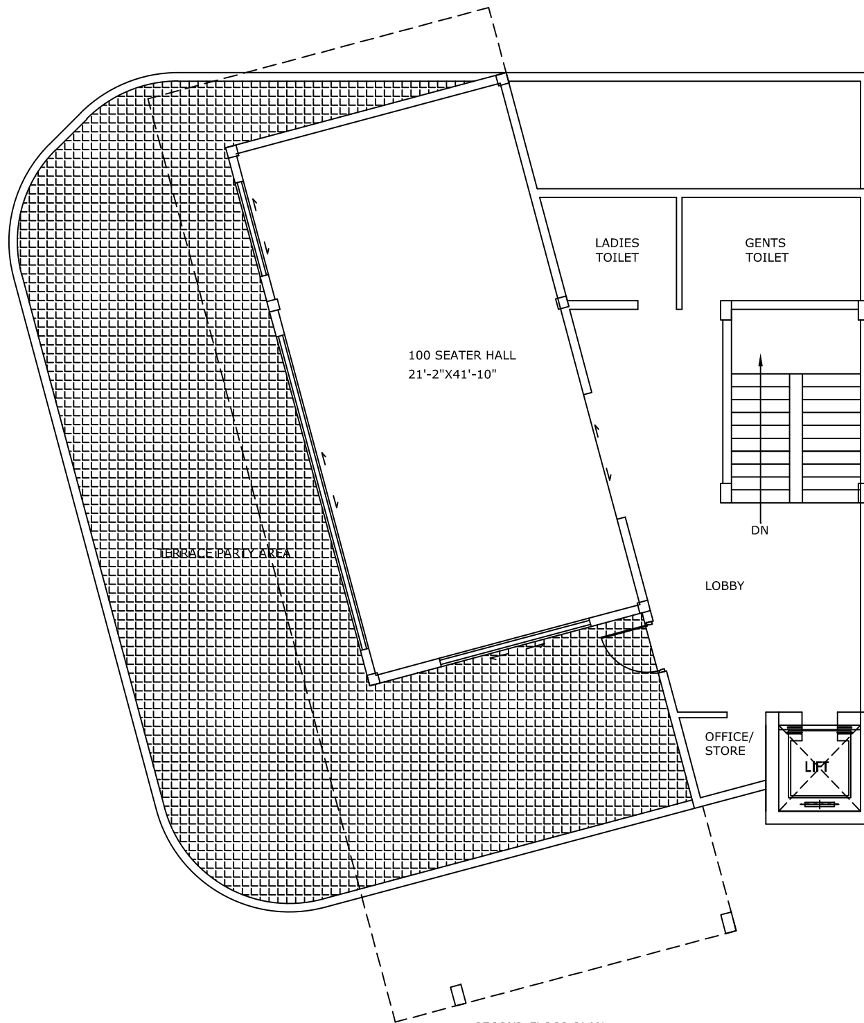
SECOND FLOOR PLAN (CLUB HOUSE)
